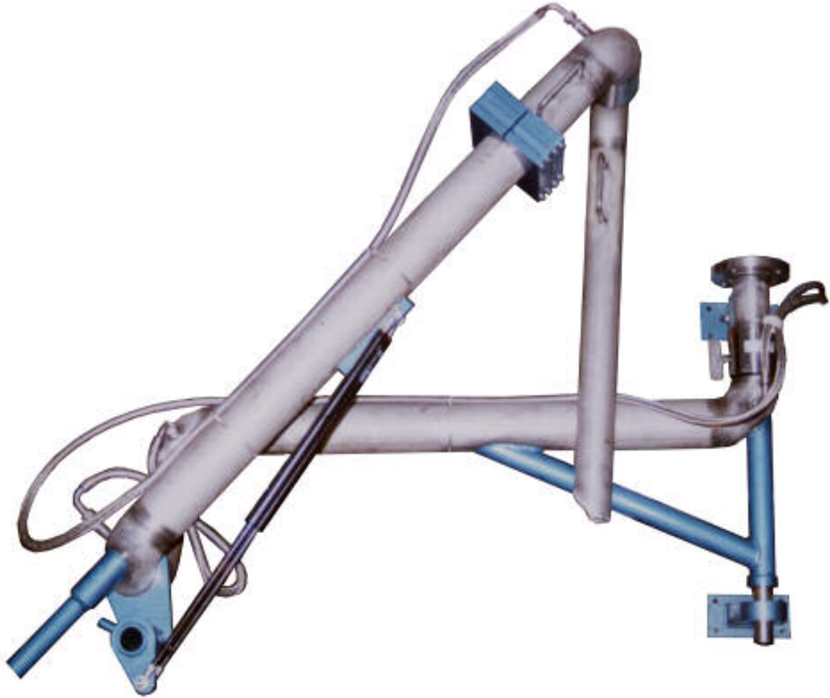
3" 316 Stainless Steel Top Loading Arm, with gas spring and steam jacketing.
